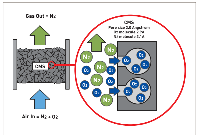
CMS Structure
